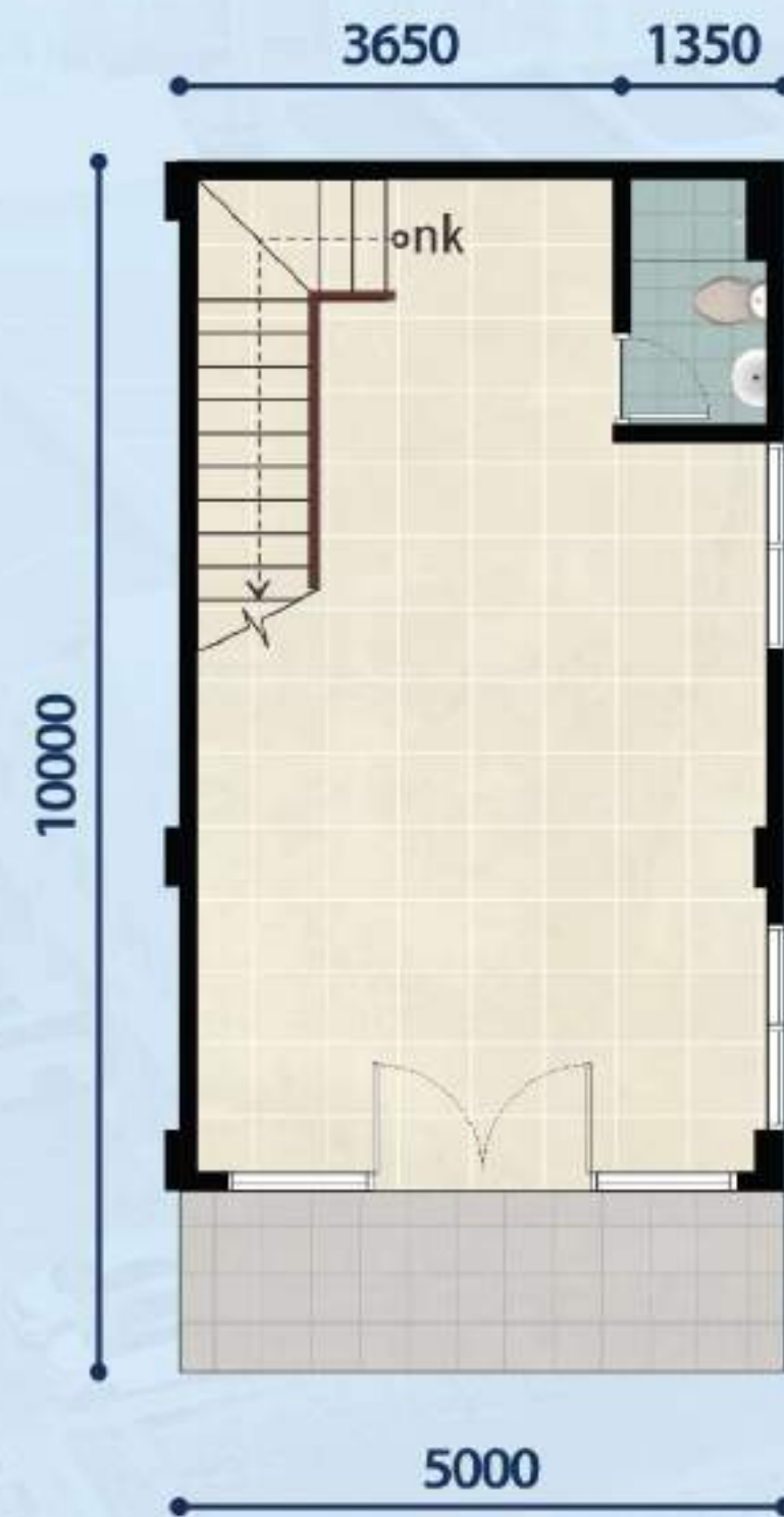
LANTAI 1
