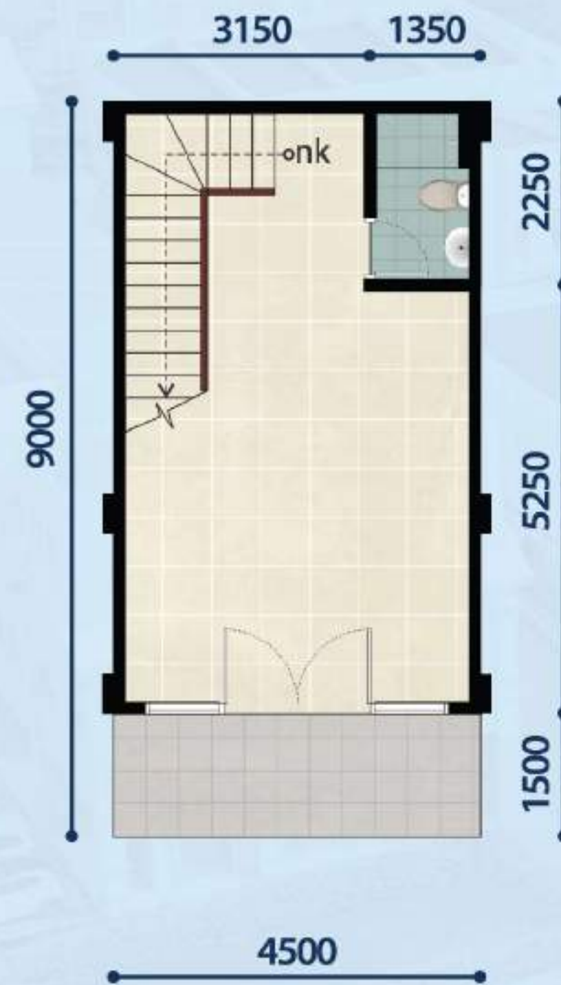
LANTAI 1
